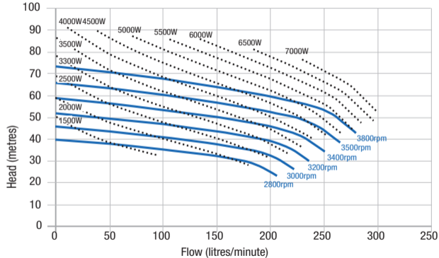
OJ800 Performance
