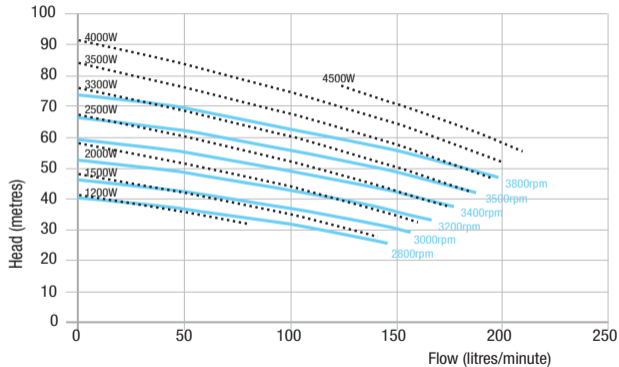
OJ700 Performance
