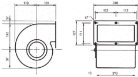
DOUBLE BLOWER
