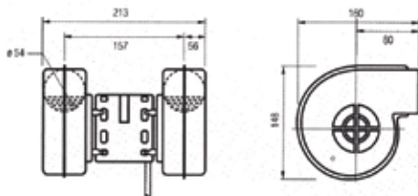
DOUBLE BLOWER
