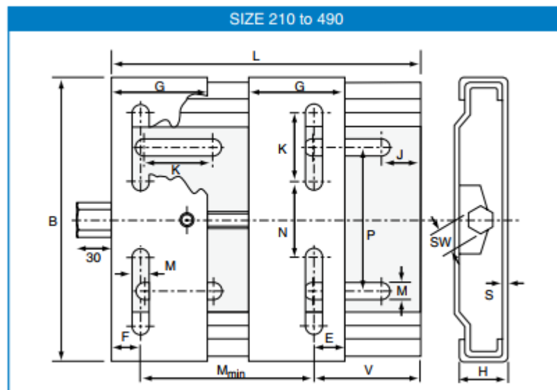
Dimensions for Sizes 210 to 490 Rapid Fit Motor Mount
