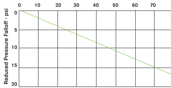
System Flow Rate - Gallon per minute (US Gal = 3.75L)
